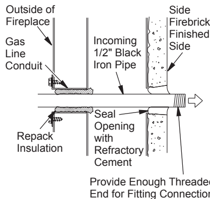
Figure 22 - Gas Line Installation
